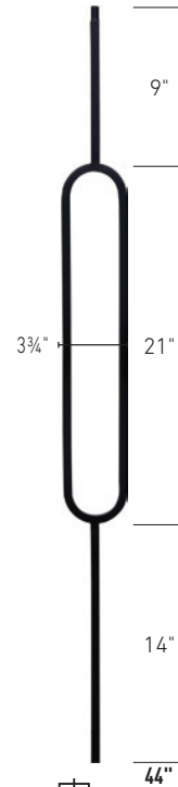
1662 44 1/2" Contempo Oval
