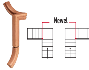
Left-hand 2 Riser With Cap
